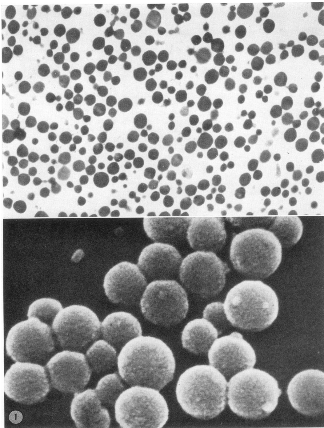
FIGURE 1 (a) Transmission electron micrograph of zymogen granules from rat pancreas. Magnification: \times 4,140 . (b) Scanning electron micrograph of a second preparation of zymogen granules. Magnification: \times 23,300 .
